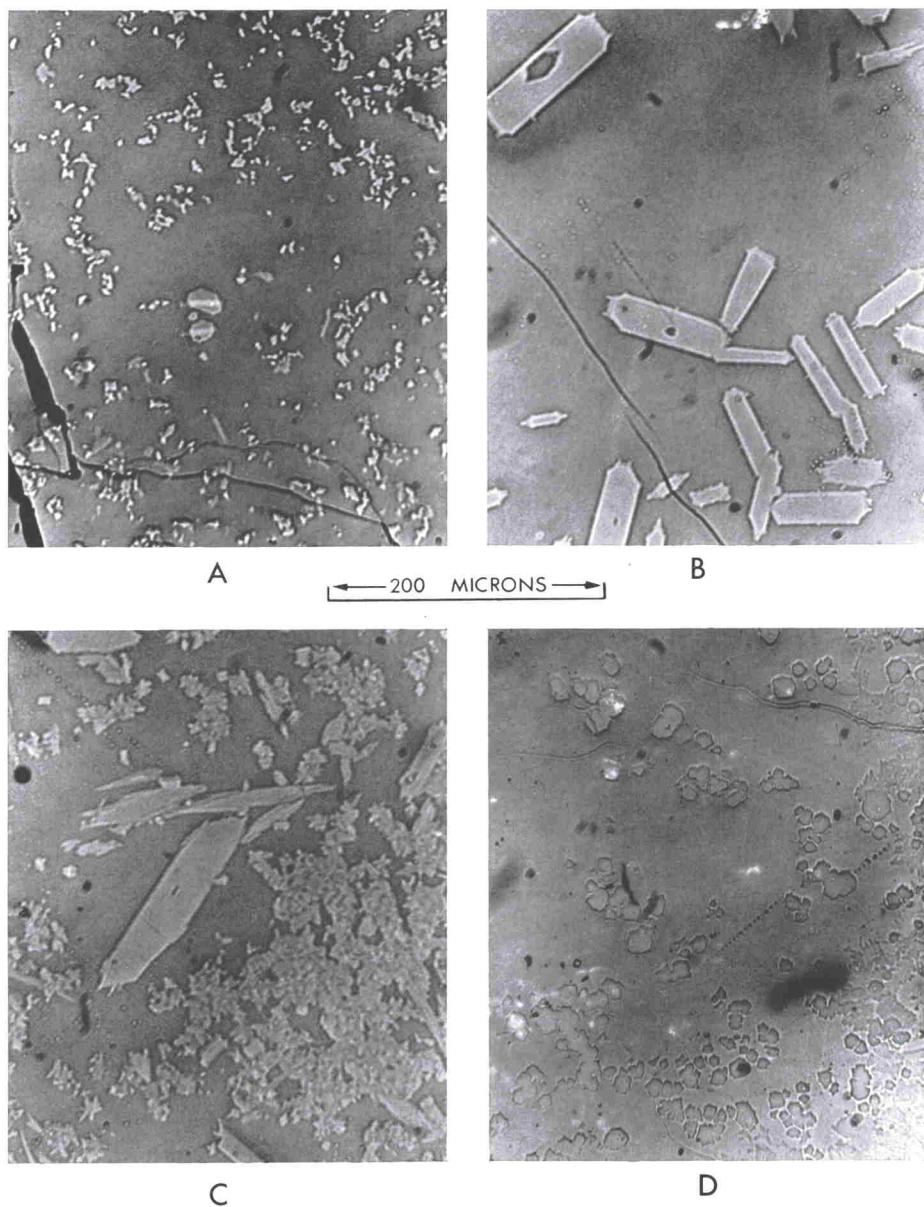
Fig. 2 A—D. Polished mounts for electron microprobe analyses showing crystalline phases in glass at various pressures. A. Olivine (small, highly reflecting grains) and orthopyroxene (larger, lath-shaped) crystals in glass. Olivine tholeiite at 9 kb, 1,290°C. White trace across larger orthopyroxenes shows path of electron beam during microprobe analyses. B. Orthopyroxene crystals in glass. Olivine tholeiite at 13.5 kb, 1380°C. Incipient nucleation of quench clinopyroxene particularly at corners of orthopyroxene. C. Large orthopyroxene and fine aggregates of quench clinopyroxene. Olivine basalt at 13.5 kb, 1,320°C. D. Garnet crystals and patchy aggregates of finegrained quench clinopyroxene (right hand side of picture) in 27 kb, 1,450°C run
